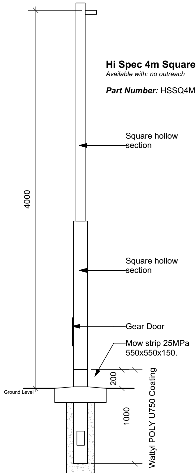
4 meter Pole (copyright Hi Spec Lighting Ltd).
